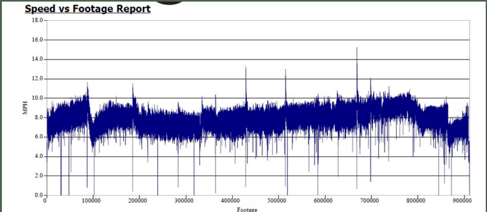
FIGURE 4 - SPEED CONTROL PIG SPEED VS FOOTAGE DATA
