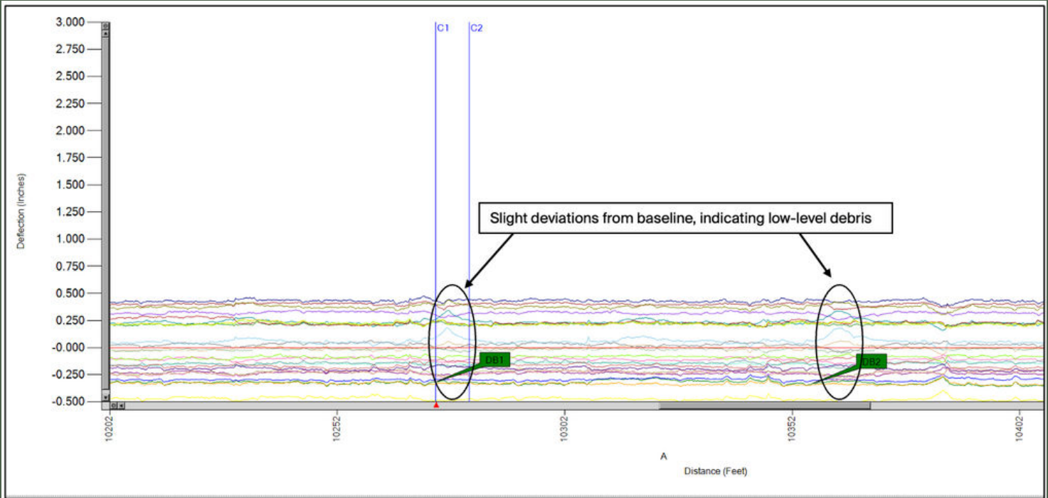
FIGURE 1 - DEBRIS MAPPING DATA
